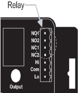
Figure 6: Relay location
