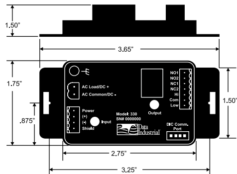
Figure 1: Dimensions
