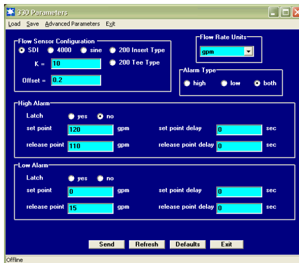
Figure 10: Parameters screen
